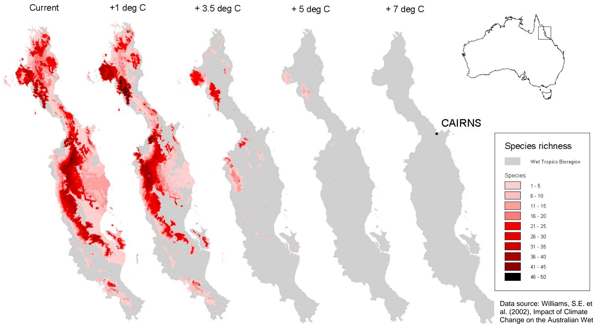
Map 11 Distribution of species richness of WT endemic terrestrial vertebrates with increasing temperature (based on BIOCLIM distribution models of each species at temperature scenario).
